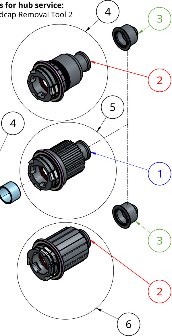
detailed freewheel explode sheet 3
